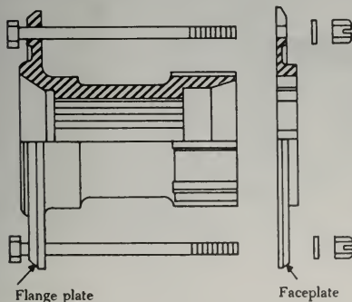
FIGURE 7-9. Hub assembly.
